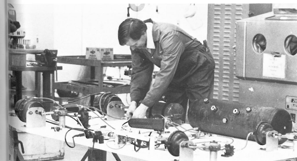
▲ Autobody students learning their skills through practical work.
